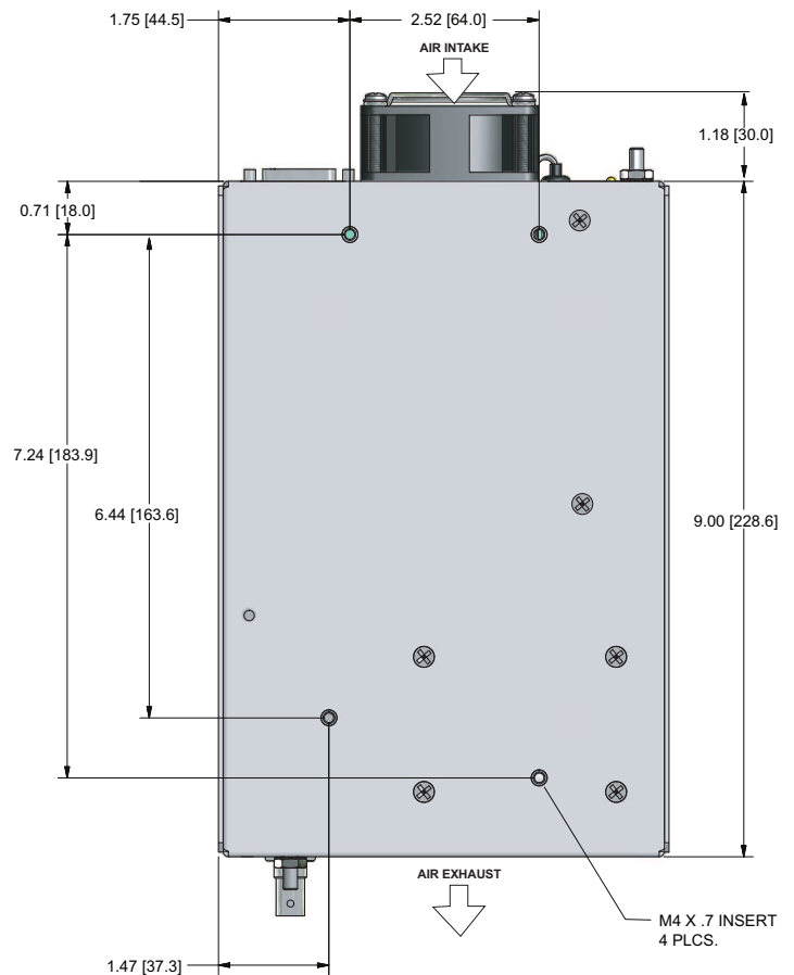
BOTTOM VIEW
