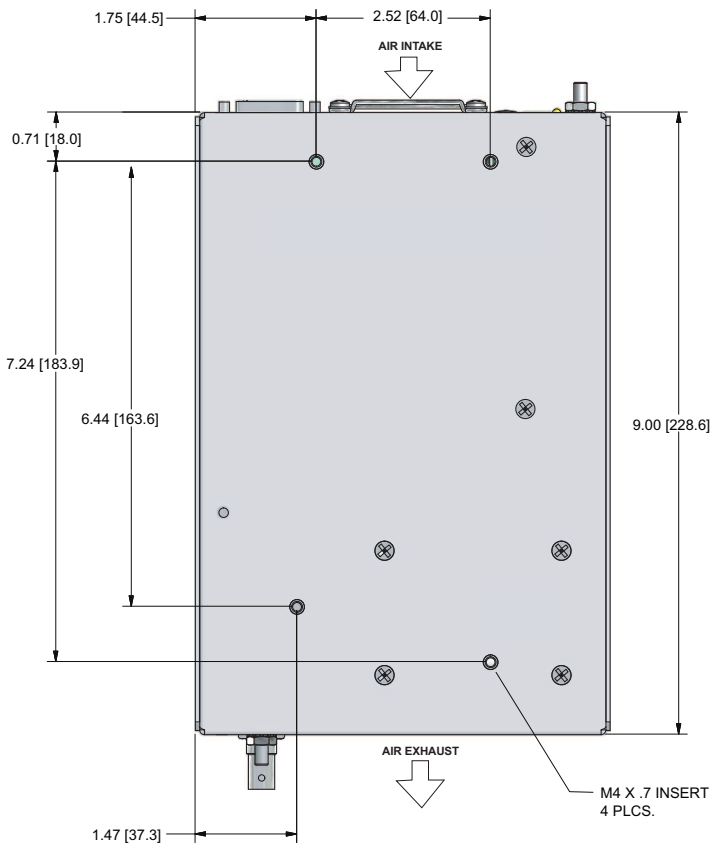
BOTTOM VIEW
